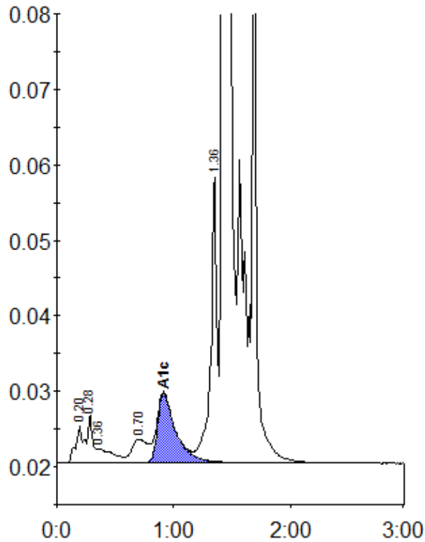
Peak table - ID: 10620257
